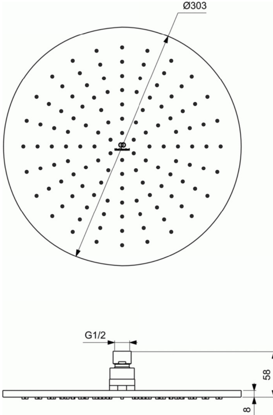
IS_Idealrain_A5803_PrListDrw_NN.eps
