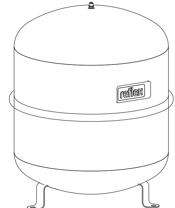
Isometric view
