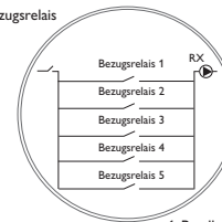
1. Parallel (OR)
