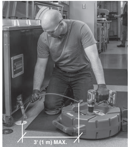
Figure 11 – In Operating Position
