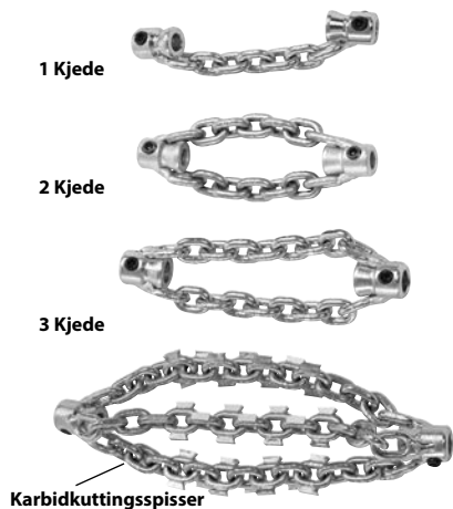
Figur 8 - Kjdebankere
