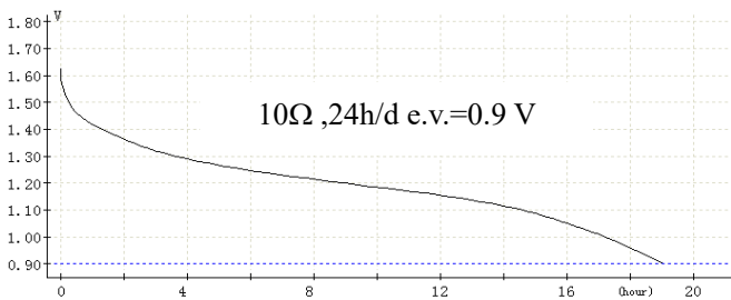
Chart 1. Discharge diagram
