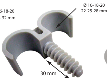
FIX-RING® Double
