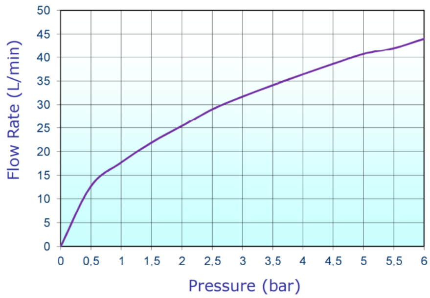
8C21011-124 flow rate (free outlet)
